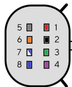
Rear view VMH Flex Molex MX150, 8 poles-connector
